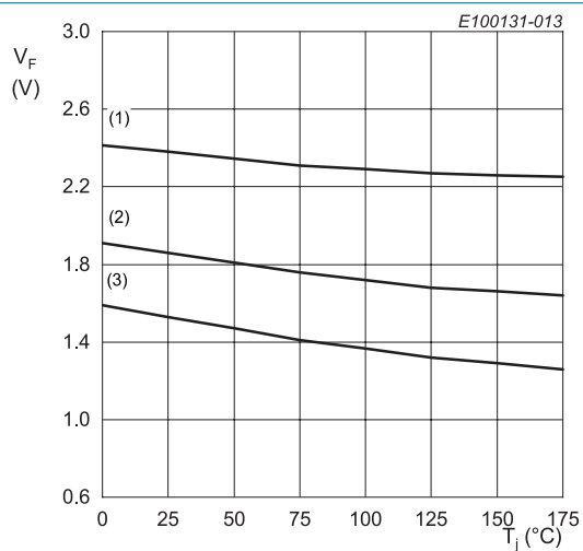
(1) I_F = 150 A (2) I_F = 75 A (3) I_F = 37.5 A Fig. 13. Typical diode forward voltage as a function of junction temperature
