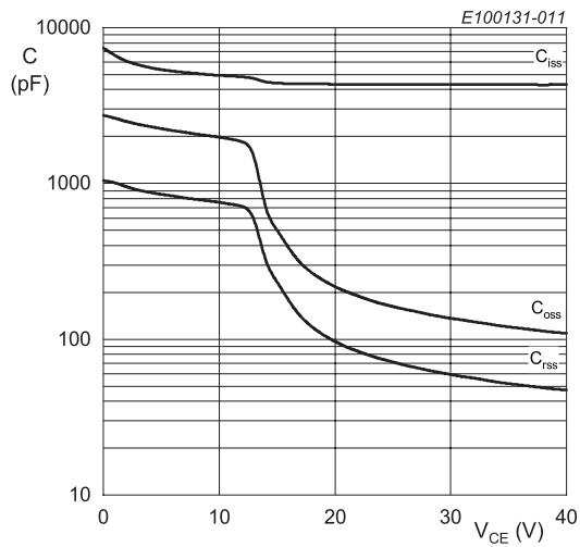
V_{GE} = 0 V; f = 1 MHz Fig. 11. Typical capacitance as a function of collector-emitter voltage
